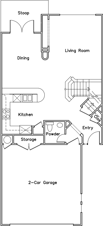
Main Level
